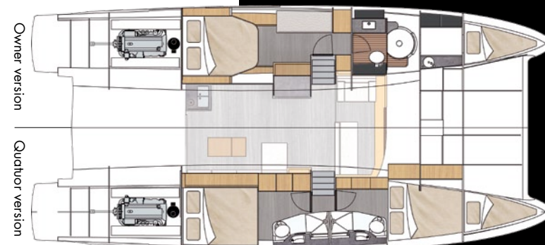
LOWER DECK
